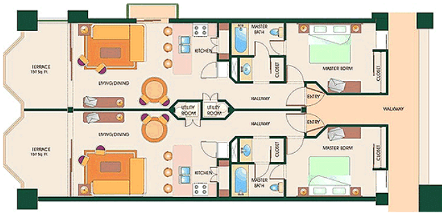
One Bedroom Floor Plan
